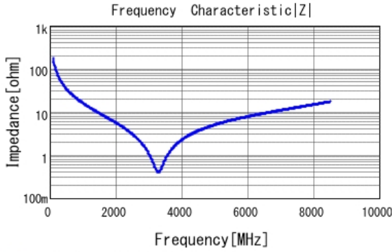
■ GRM0335C1H9R0BA01 |Z| DCOV, 25degC
