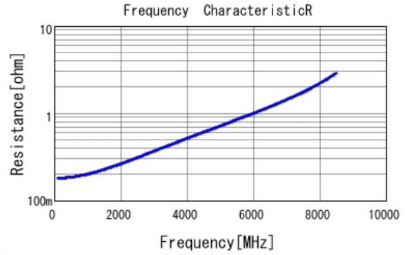
■ GRM0335C1H9R0BA01 R DCOV, 25degC
