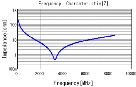
■ GRM0335C1H9R0CA01 |Z| DCOV, 25degC
