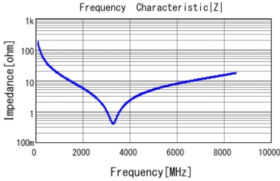
■ GRM0335C1H9R0DA01 |Z| DCOV, 25degC
