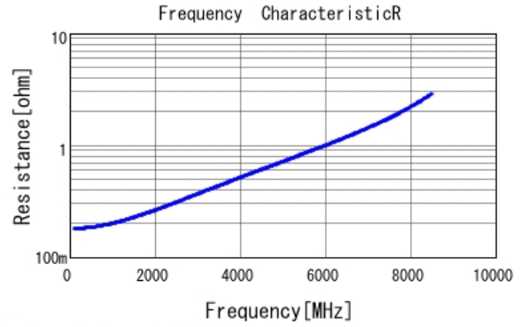
■ GRM0335C1H9R0DA01 R DCOV, 25degC
