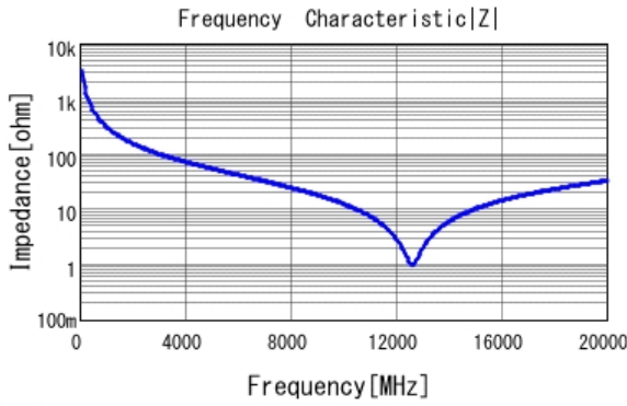
■ GRM0335C1HR50BA01 |Z| DCOV, 25degC
