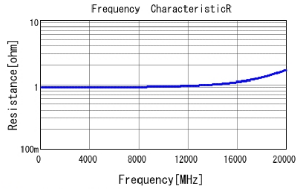
■ GRM0335C1HR50BA01 R DCOV, 25degC
