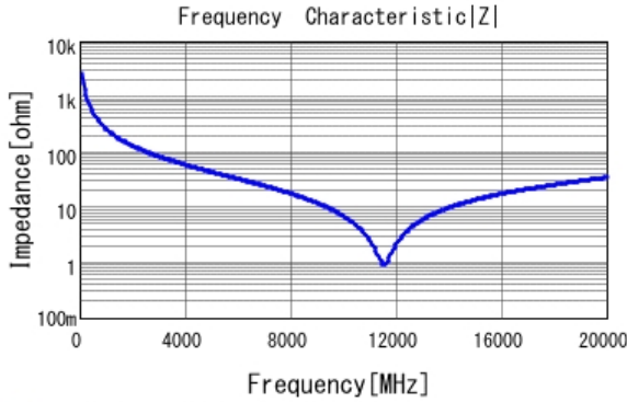
■ GRM0335C1HR60BA01 |Z| DCOV, 25degC
