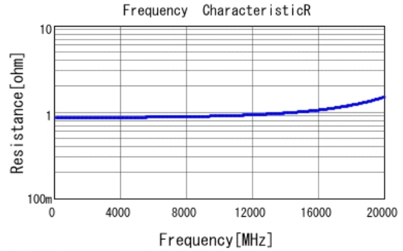
■ GRM0335C1HR60BA01 R DCOV, 25degC
