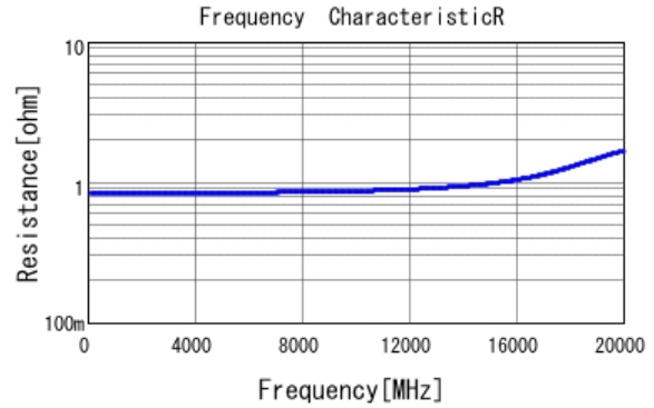
■ GRM0335C1HR70BA01 R DCOV, 25degC
