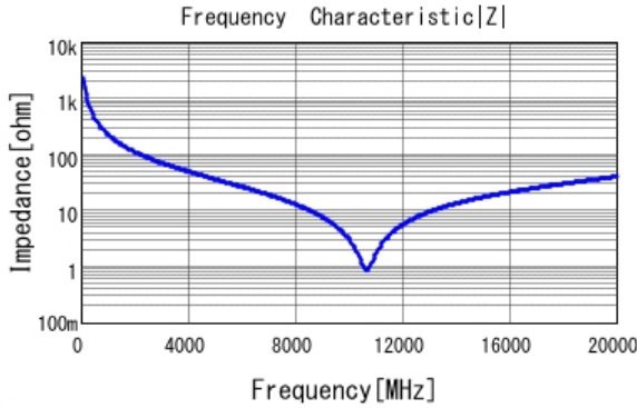
■ GRM0335C1HR70BA01 |Z| DCOV, 25degC
