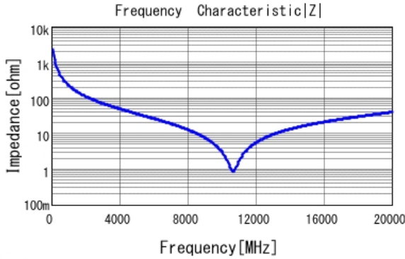
■ GRM0335C1HR70WA01 |Z| DCOV, 25degC
