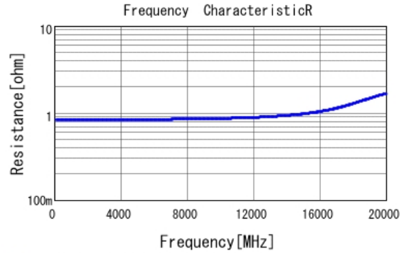
■ GRM0335C1HR70WA01 R DCOV, 25degC
