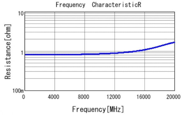
■ GRM0335C1HR80BA01 R DCOV, 25degC
