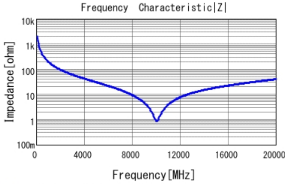
■ GRM0335C1HR80BA01 |Z| DCOV, 25degC
