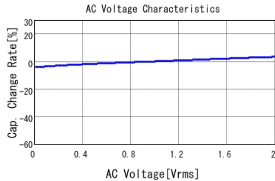
■ GRM033B11C681KA01 C-AC Voltage capchange, DCOV, 20.0d
