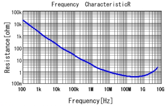
■ GRM033B11C681KA01 R DCOV, 20degC
