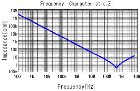
■ GRM033B11C681KA01 |Z| DCOV, 20degC
