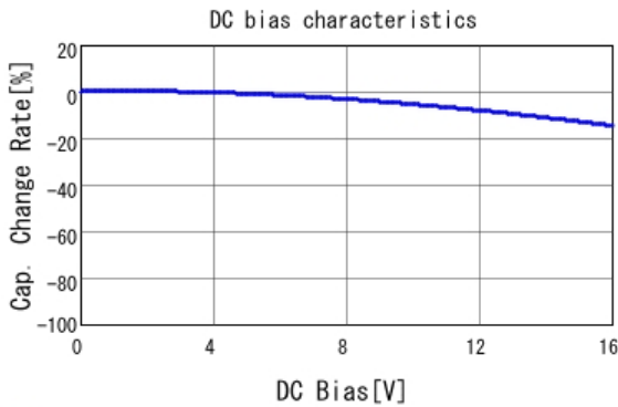
■ GRM033B11C681KA01 C-DC bias capchange, 20.0degC, AC1.
