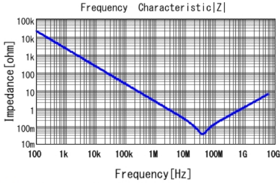
■ GRM033C71A104KE14 |Z| DCOV, 25degC
