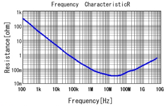
■ GRM033C71A104KE14 R DCOV, 25degC
