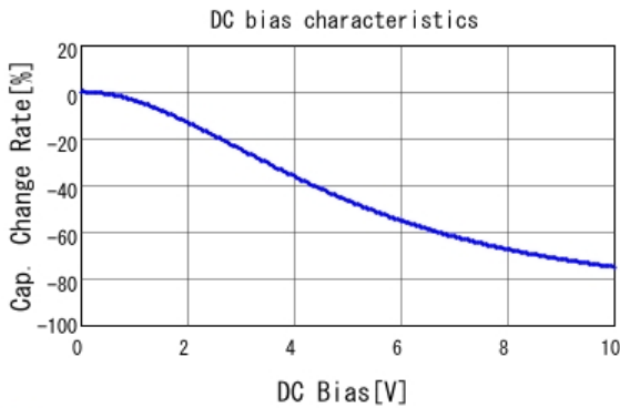
■ GRM033C71A104KE14 C-DC bias capchange, 25.0degC, AC1V
