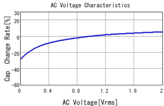
■ GRM033C71C104KE14 C-AC Voltage capchange, DCOV, 25.0d
