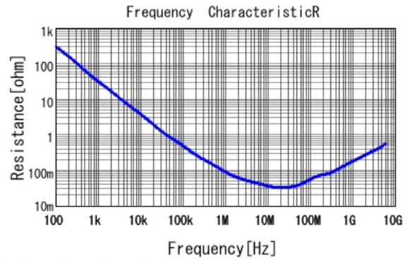
■ GRM033C71C104KE14 R DCOV, 25degC
