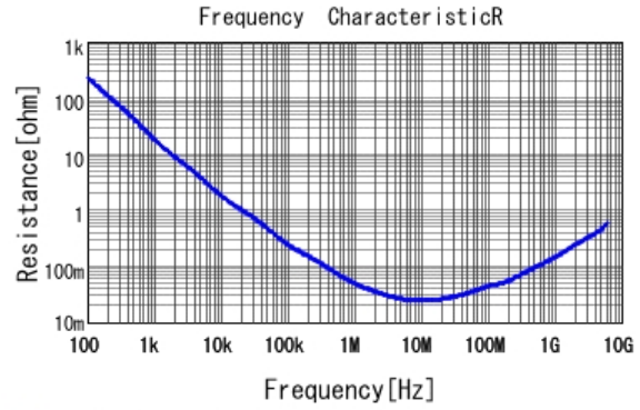
■ GRM033C80J104KE15 R DCOV, 25degC
