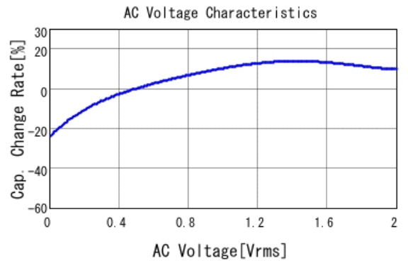
■ GRM033C80J104KE15 C-AC Voltage capchange, DCOV, 25.0d
