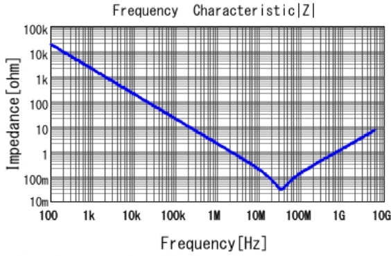
■ GRM033C80J104KE15 |Z| DCOV, 25degC
