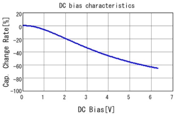
■ GRM033C80J104KE15 C-DC bias capchange, 25.0degC, AC0.
