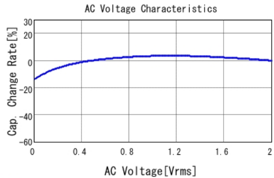
■ GRM033C80J105ME05 C-AC Voltage capchange, DCOV, 25.0d
