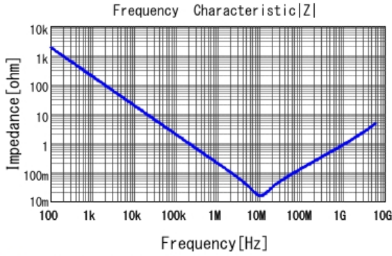
■ GRM033C80J105ME05 |Z| DCOV, 25degC
