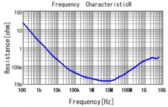
■ GRM033C80J105ME05 R DCOV, 25degC
