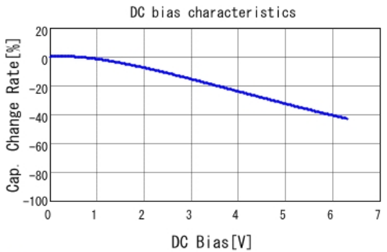
■ GRM033C80J473KE19 C-DC bias capchange, 25.0degC, AC0.
