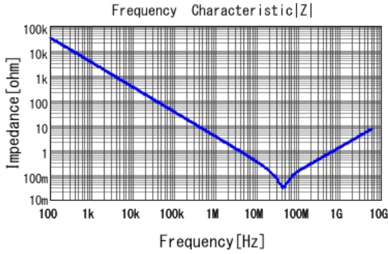
■ GRM033C80J473KE19 |Z| DCOV, 25degC
