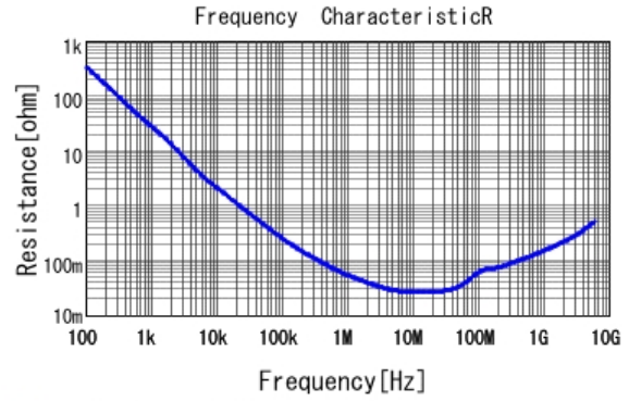
■ GRM033C80J473KE19 R DCOV, 25degC
