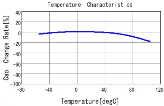
■ GRM033C80J473KE19 C-Temp. capchange, DC0.0V, AC0.5Vrm
