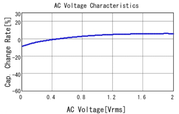
■ GRM033C80J473KE19 C-AC Voltage capchange, DCOV, 25.0d
