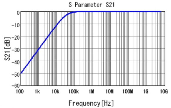
■ GRM033C80J473KE19 S21 DC0V, 25degC
