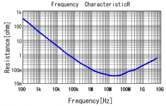
■ GRM033C81C104KE14 R DCOV, 25degC
