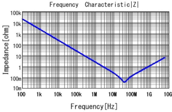
■ GRM033C81C104KE14 |Z| DCOV, 25degC
