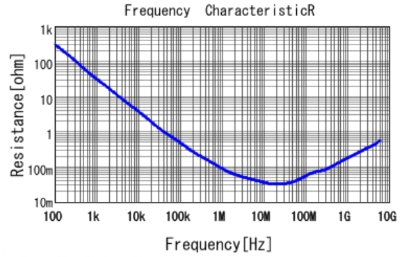
■ GRM033C81E104KE14 R DCOV, 25degC
