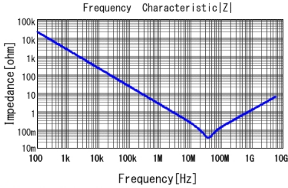
■ GRM033C81E104KE14 |Z| DCOV, 25degC
