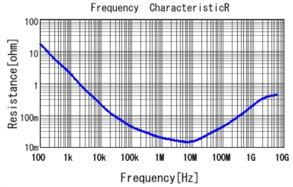
■ GRM033D70J105ME01 R DCOV, 25degC
