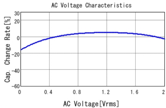
■ GRM033D70J105ME01 C-AC Voltage capchange, DCOV, 25.0d
