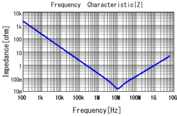
■ GRM033D70J105ME01 |Z| DCOV, 25degC
