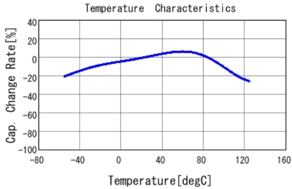
■ GRM033D70J105ME01 C-Temp. capchange, DC0.0V, AC0.02Vr
