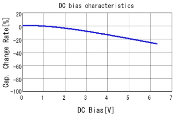
■ GRM033R60J223KE01 C-DC bias capchange, 25.0degC, AC0.
