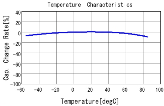
■ GRM033R60J223KE01 C-Temp. capchange, DC0.0V, AC0.5Vrm
