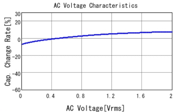
■ GRM033R60J223KE01 C-AC Voltage capchange, DCOV, 25.0d
