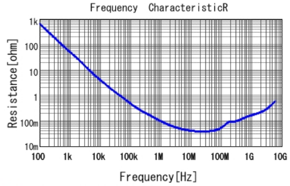
■ GRM033R60J223KE01 R DCOV, 25degC
