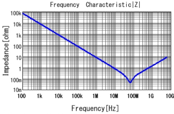
■ GRM033R60J223KE01 |Z| DCOV, 25degC
