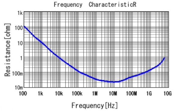
■ GRM033R60J224KE15 R DCOV, 25degC
