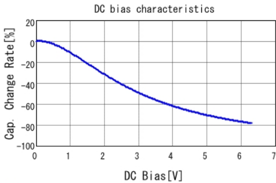
■ GRM033R60J224KE15 C-DC bias capchange, 25.0degC, AC0.
