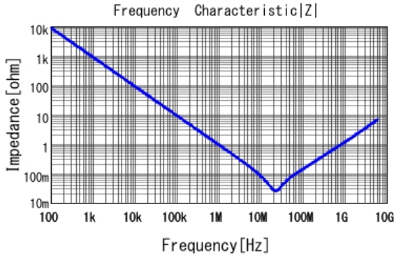
■ GRM033R60J224KE15 |Z| DCOV, 25degC
