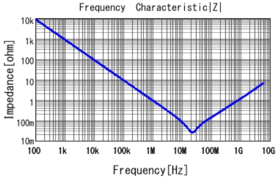
■ GRM033R60J224ME15 |Z| DCOV, 25degC
