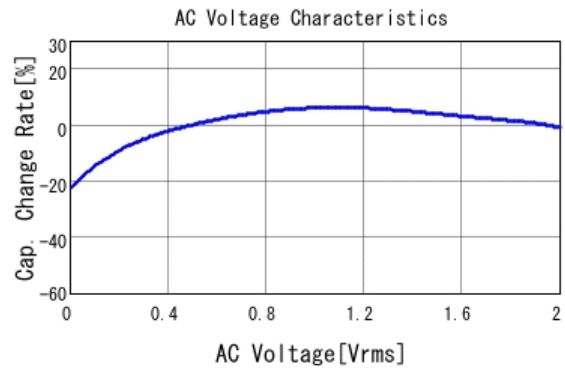
■ GRM033R60J224ME15 C-AC Voltage capchange, DCOV, 25.0d
