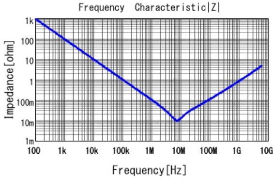
■ GRM033R60J225ME15 |Z| DCOV, 25degC
