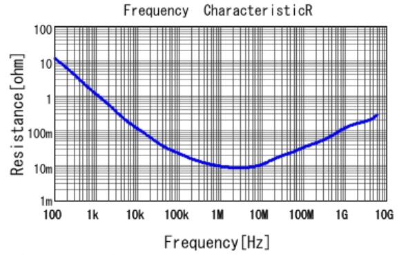
■ GRM033R60J225ME15 R DCOV, 25degC
