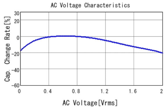
■ GRM033R60J225ME15 C-AC Voltage capchange, DCOV, 25.0d
