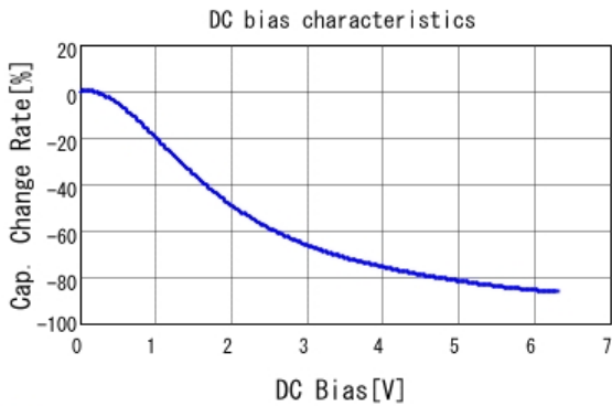
■ GRM033R60J225ME15 C-DC bias capchange, 25.0degC, AC0.
