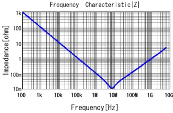
■ GRM033R60J225ME47 |Z| DCOV, 25degC
