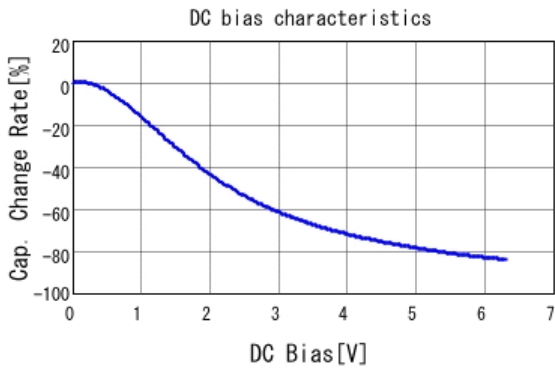
■ GRM033R60J225ME47 C-DC bias capchange, 25.0degC, AC0.
