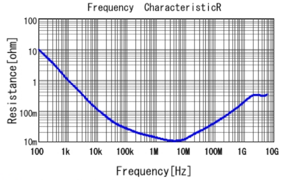
■ GRM033R60J225ME47 R DCOV, 25degC
