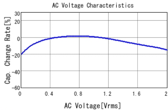
■ GRM033R60J225ME47 C-AC Voltage capchange, DCOV, 25.0d
