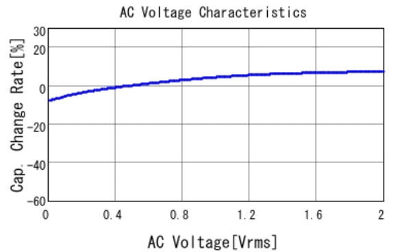
■ GRM033R60J333KE01 C-AC Voltage capchange, DCOV, 25.0d
