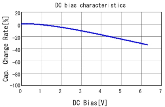
■ GRM033R60J333KE01 C-DC bias capchange, 25.0degC, AC0.
