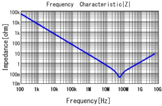
■ GRM033R60J333KE01 |Z| DCOV, 25degC
