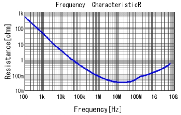
■ GRM033R60J333KE01 R DCOV, 25degC
