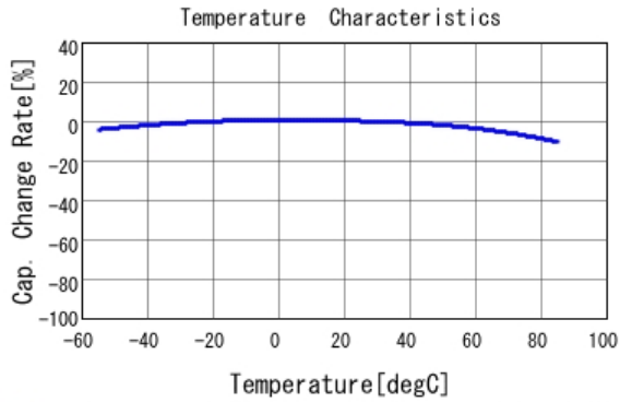
■ GRM033R60J473KE19 C-Temp. capchange, DC0.0V, AC0.5V rm
