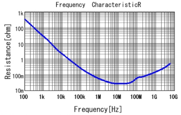
■ GRM033R60J473KE19 R DCOV, 25degC
