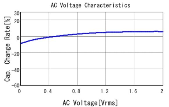
■ GRM033R60J473KE19 C-AC Voltage capchange, DCOV, 25.0d
