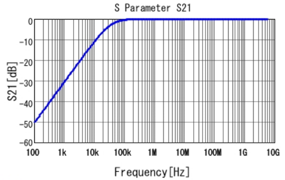
■ GRM033R60J473KE19 S21 DC0V, 25degC
