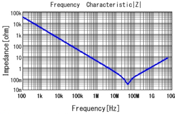
■ GRM033R60J473KE19 |Z| DCOV, 25degC
