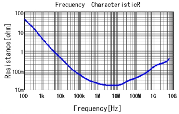
■ GRM033R60J474KE90 R DCOV, 25degC
