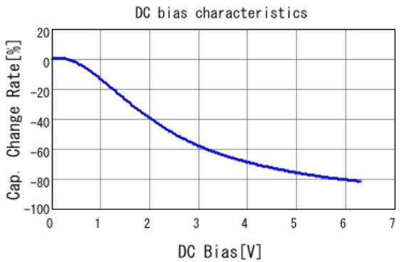
■ GRM033R60J474KE90 C-DC bias capchange, 25.0degC, AC0.
