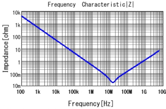
■ GRM033R60J474KE90 |Z| DCOV, 25degC
