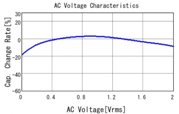
■ GRM033R60J474KE90 C-AC Voltage capchange, DCOV, 25.0d
