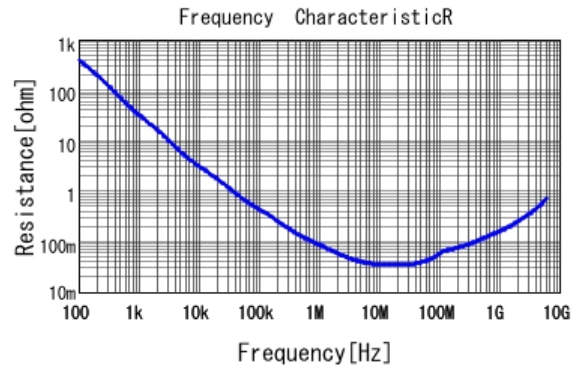
■ GRM033R60J683KE19 R DCOV, 25degC
