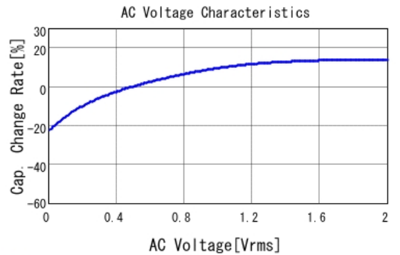
■ GRM033R60J683KE19 C-AC Voltage capchange, DCOV, 25.0d
