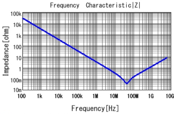
■ GRM033R60J683KE19 |Z| DCOV, 25degC
