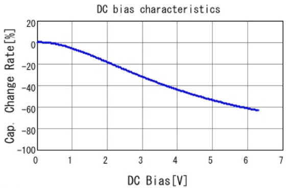
■ GRM033R60J683KE19 C-DC bias capchange, 25.0degC, AC0.
