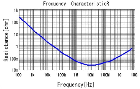
■ GRM033R61A104KE15 R DCOV, 25degC
