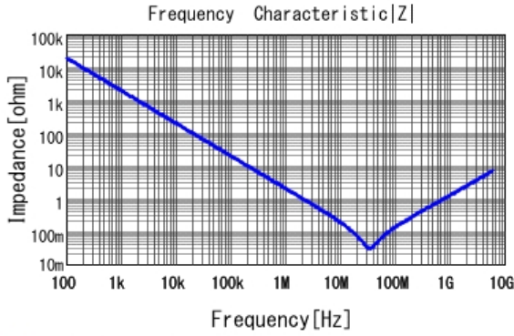
■ GRM033R61A104KE15 |Z| DCOV, 25degC
