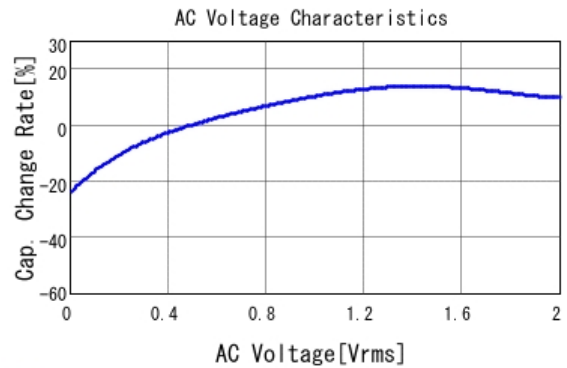
■ GRM033R61A104KE15 C-AC Voltage capchange, DCOV, 25.0d
