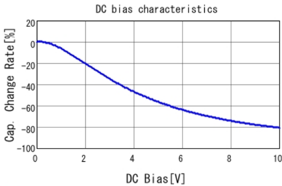
■ GRM033R61A104KE15 C-DC bias capchange, 25.0degC, AC0.
