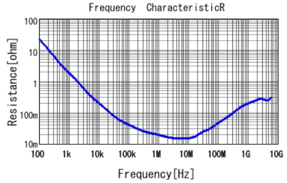
■ GRM033R61A105ME15 R DCOV, 25degC
