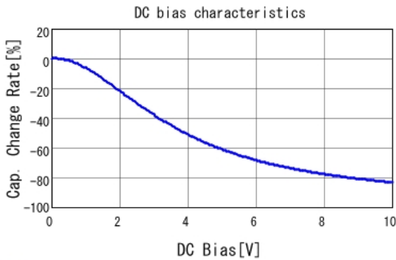
■ GRM033R61A105ME15 C-DC bias capchange, 25.0degC, AC1V
