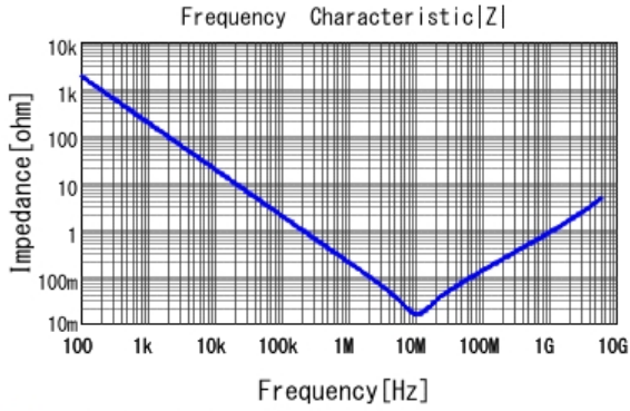
■ GRM033R61A105ME15 |Z| DCOV, 25degC
