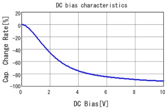
■ GRM033R61A105ME44 C-DC bias capchange, 25.0degC, AC1V
