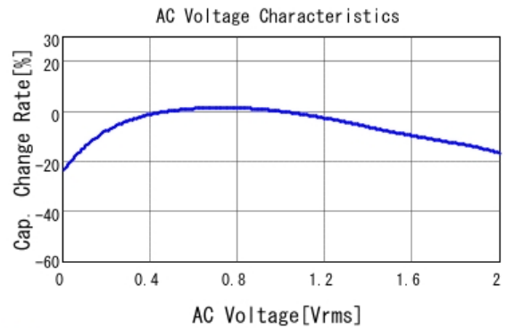
■ GRM033R61A105ME44 C-AC Voltage capchange, DCOV, 25.0d
