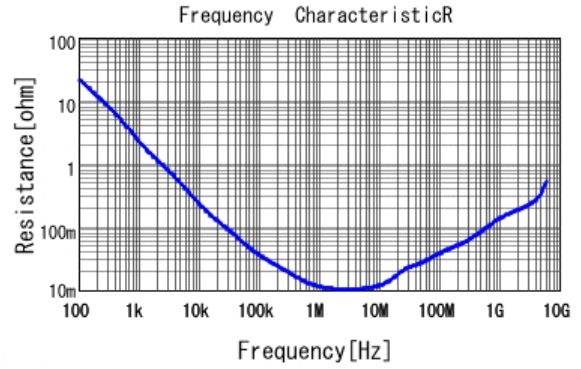
■ GRM033R61A105ME44 R DCOV, 25degC
