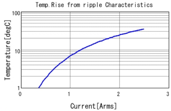
■ GRM033R61A105ME44 Temp. rise 1MHz
