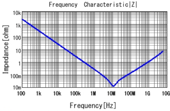
■ GRM033R61A105ME44 |Z| DCOV, 25degC
