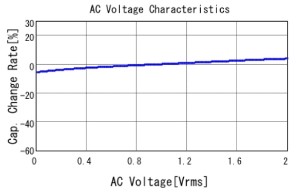
■ GRM033R61A182KA01 C-AC Voltage capchange, DCOV, 25.0d
