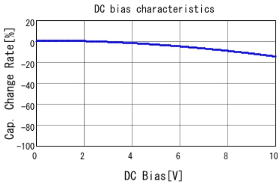
■ GRM033R61A182KA01 C-DC bias capchange, 25.0degC, AC1.
