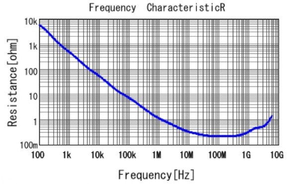
■ GRM033R61A182KA01 R DCOV, 25degC
