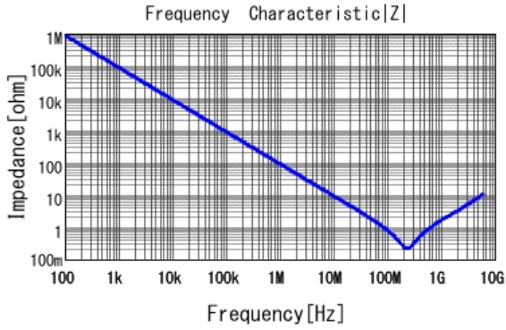
■ GRM033R61A182KA01 |Z| DCOV, 25degC
