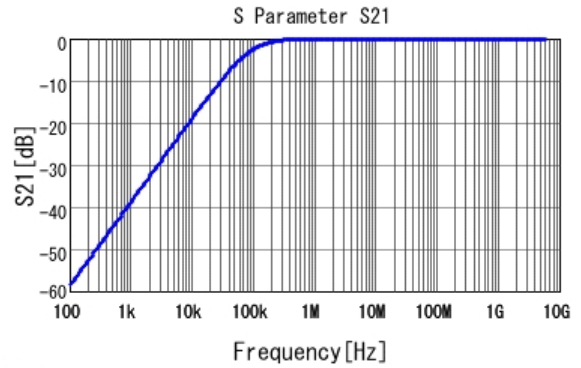
■ GRM033R61A183KE84 S21 DC0V, 25degC
