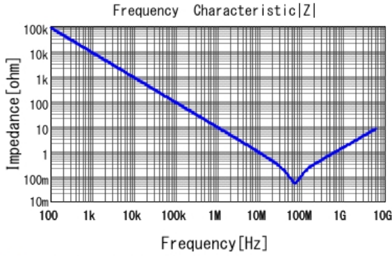
■ GRM033R61A183KE84 |Z| DCOV, 25degC
