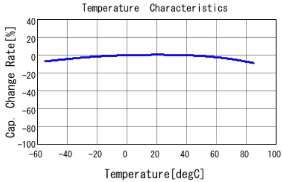
■ GRM033R61A183KE84 C-Temp. capchange, DC0.0V, AC0.5Vrm
