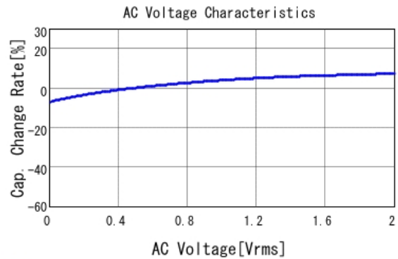
■ GRM033R61A183KE84 C-AC Voltage capchange, DCOV, 25.0d
