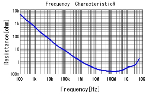
■ GRM033R61A222KA01 R DCOV, 25degC
