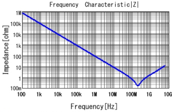
■ GRM033R61A222KA01 |Z| DCOV, 25degC
