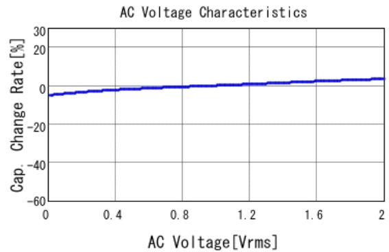
■ GRM033R61A222KA01 C-AC Voltage capchange, DCOV, 25.0d
