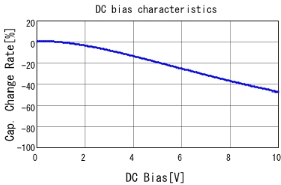
■ GRM033R61A223KE84 C-DC bias capchange, 25.0degC, AC0.
