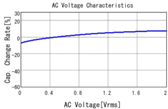
■ GRM033R61A223KE84 C-AC Voltage capchange, DCOV, 25.0d
