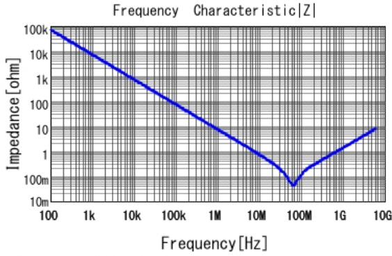
■ GRM033R61A223KE84 |Z| DCOV, 25degC
