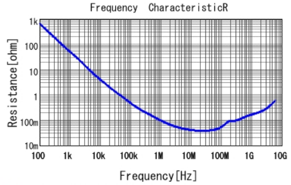
■ GRM033R61A223KE84 R DCOV, 25degC
