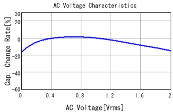
■ GRM033R61A225KE47 C-AC Voltage capchange, DCOV, 25.0d
