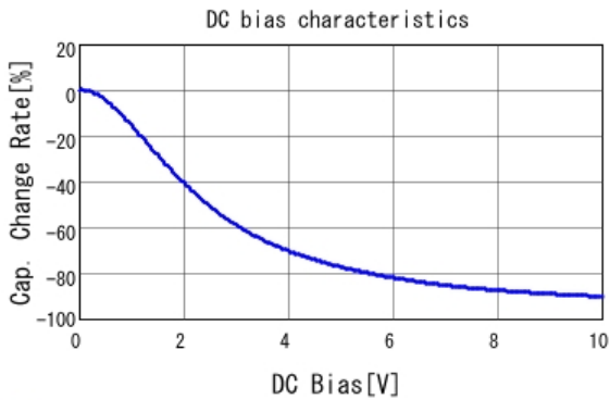
■ GRM033R61A225KE47 C-DC bias capchange, 25.0degC, AC1V
