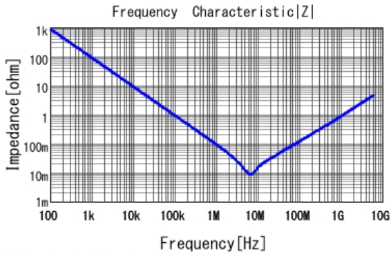
■ GRM033R61A225KE47 |Z| DCOV, 25degC
