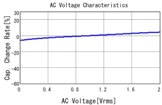
■ GRM033R61A332KA01 C-AC Voltage capchange, DCOV, 25.0d
