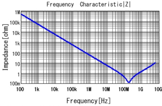
■ GRM033R61A332KA01 |Z| DCOV, 25degC
