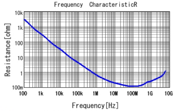
■ GRM033R61A332KA01 R DCOV, 25degC
