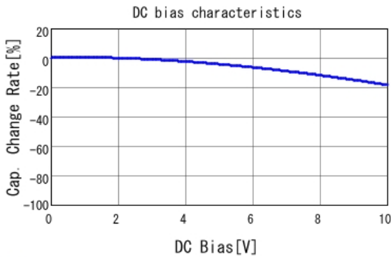
■ GRM033R61A332KA01 C-DC bias capchange, 25.0degC, AC1.
