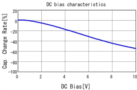
■ GRM033R61A333KE84 C-DC bias capchange, 25.0degC, AC0.
