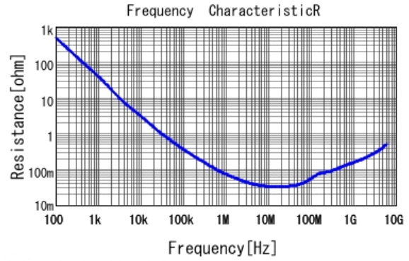
■ GRM033R61A333KE84 R DCOV, 25degC
