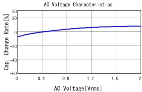
■ GRM033R61A333KE84 C-AC Voltage capchange, DCOV, 25.0d
