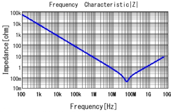
■ GRM033R61A333KE84 |Z| DCOV, 25degC
