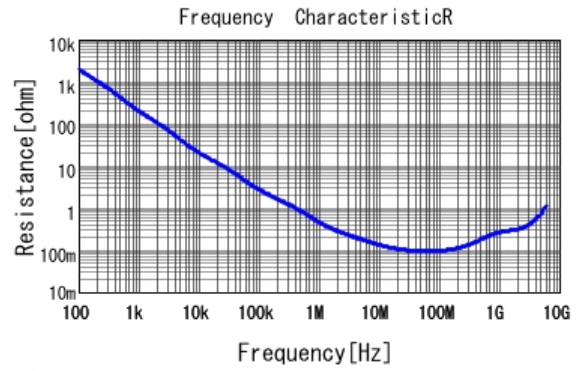
■ GRM033R61A472KA01 R DCOV, 25degC
