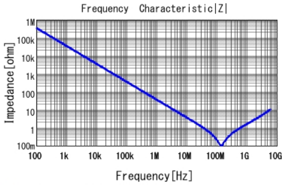
■ GRM033R61A472KA01 |Z| DCOV, 25degC
