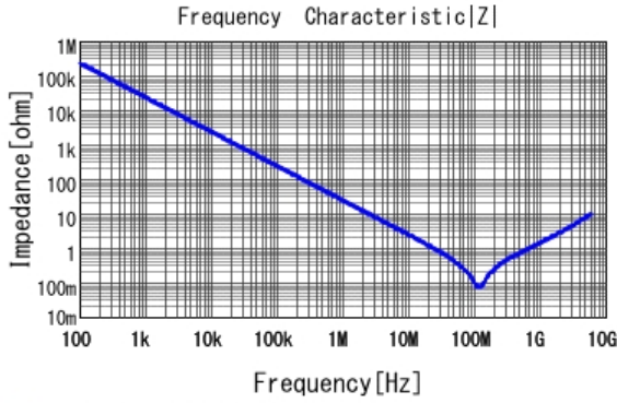
■ GRM033R61A682KA01 |Z| DCOV, 25degC
