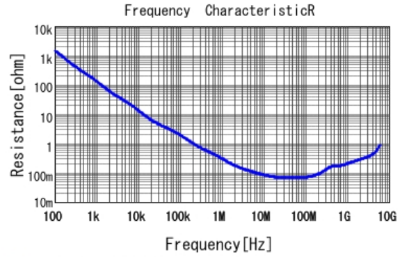
■ GRM033R61A682KA01 R DCOV, 25degC
