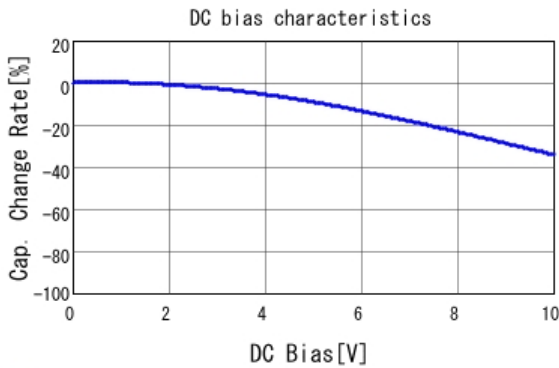
■ GRM033R61A682KA01 C-DC bias capchange, 25.0degC, AC1.
