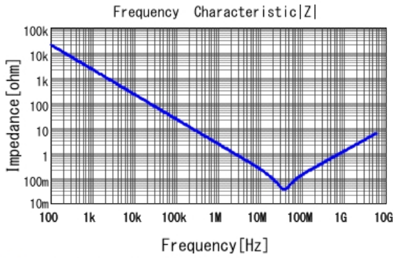
■ GRM033R61C104KE14 |Z| DCOV, 25degC
