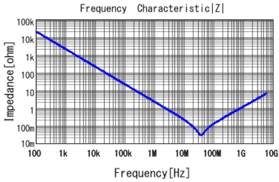
■ GRM033R61C104KE18 |Z| DCOV, 25degC
