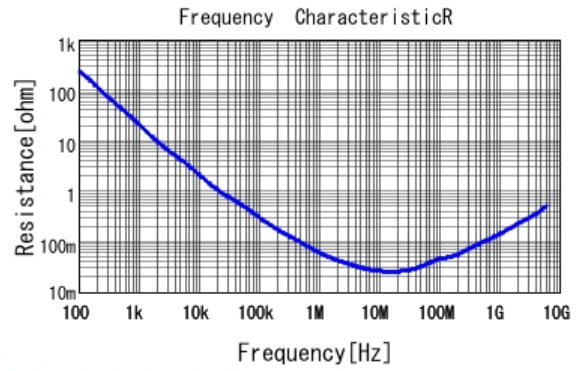
■ GRM033R61C104KE18 R DCOV, 25degC
