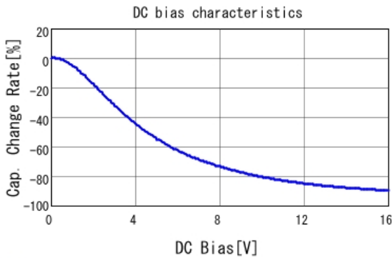
■ GRM033R61C104KE18 C-DC bias capchange, 25.0degC, AC1V
