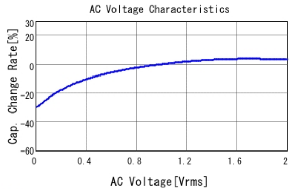
■ GRM033R61C104KE18 C-AC Voltage capchange, DCOV, 25.0d
