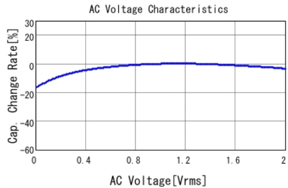
■ GRM033R61C105ME15 C-AC Voltage capchange, DCOV, 25.0d
