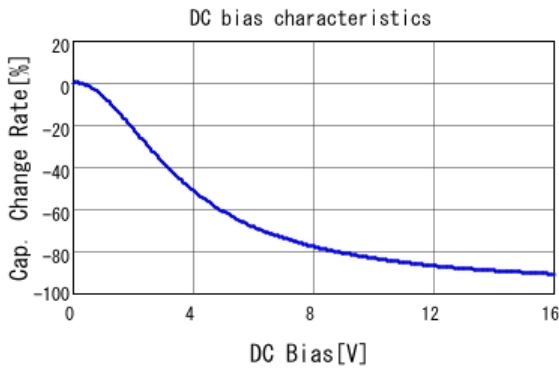
■ GRM033R61C105ME15 C-DC bias capchange, 25.0degC, AC1V
