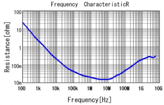
■ GRM033R61C105ME15 R DCOV, 25degC
