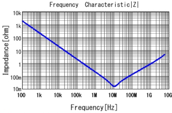
■ GRM033R61C105ME15 |Z| DCOV, 25degC
