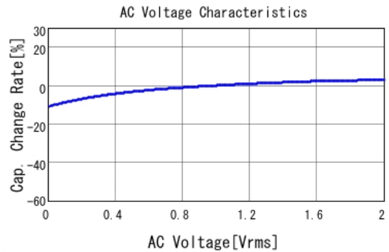
■ GRM033R61C333KE84 C-AC Voltage capchange, DCOV, 25.0d
