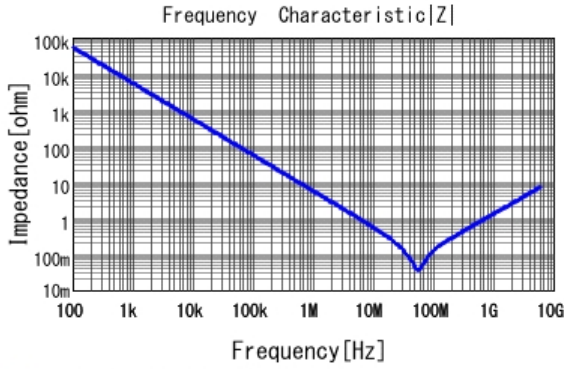
■ GRM033R61C333KE84 |Z| DCOV, 25degC
