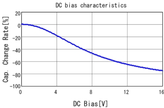
■ GRM033R61C333KE84 C-DC bias capchange, 25.0degC, AC1.
