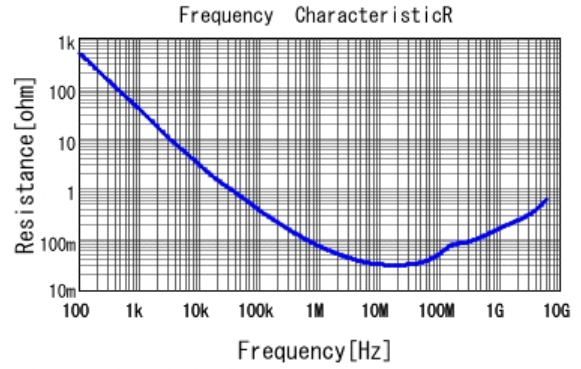
■ GRM033R61C333KE84 R DCOV, 25degC
