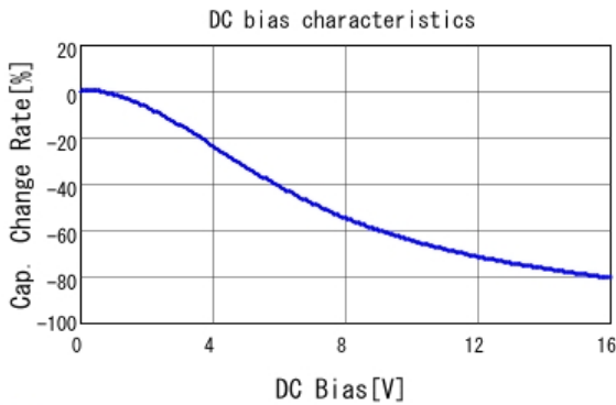
■ GRM033R61C473KE84 C-DC bias capchange, 25.0degC, AC1.
