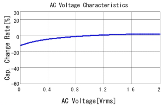
■ GRM033R61C473KE84 C-AC Voltage capchange, DCOV, 25.0d
