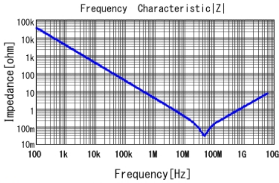
■ GRM033R61C473KE84 |Z| DCOV, 25degC
