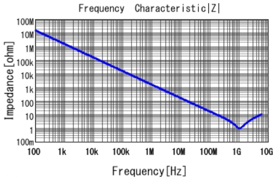
■ GRM033R61E101KA01 |Z| DCOV, 25degC
