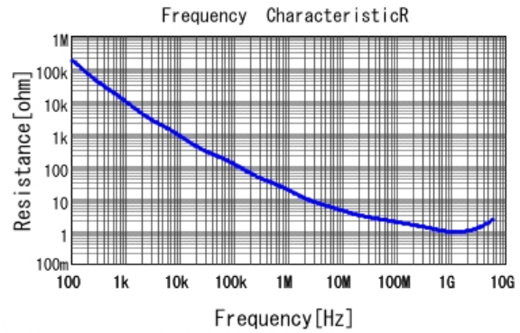
■ GRM033R61E101KA01 R DCOV, 25degC
