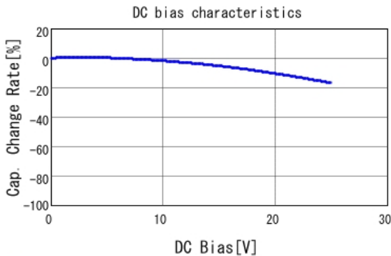
■ GRM033R61E101KA01 C-DC bias capchange, 25.0degC, AC1.
