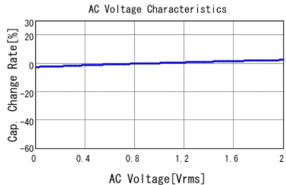
■ GRM033R61E101KA01 C-AC Voltage capchange, DCOV, 25.0d
