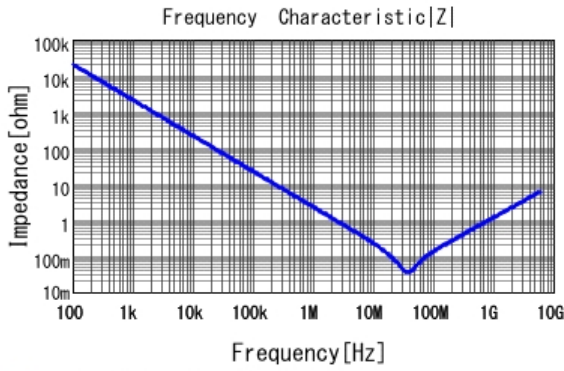
■ GRM033R61E104KE14 |Z| DCOV, 25degC
