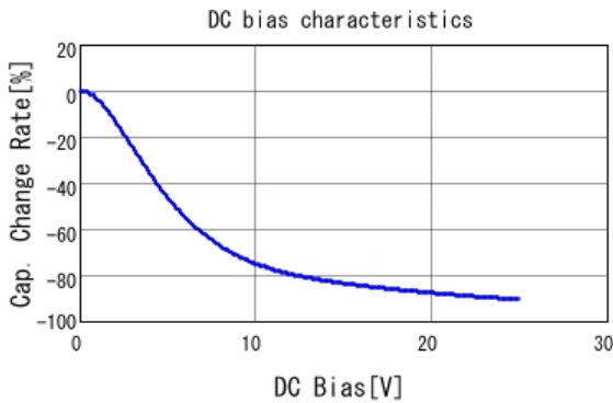
■ GRM033R61E104KE14 C-DC bias capchange, 25.0degC, AC1V
