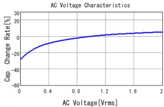
■ GRM033R61E104KE14 C-AC Voltage capchange, DCOV, 25.0d
