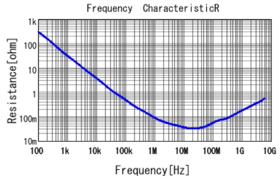
■ GRM033R61E104KE14 R DCOV, 25degC
