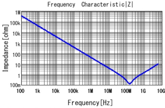
■ GRM033R61E472KA12 |Z| DCOV, 25degC
