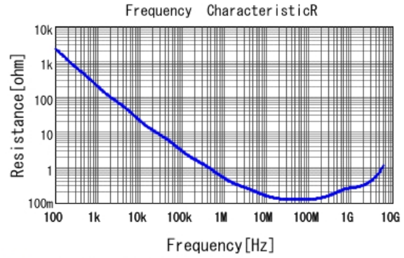
■ GRM033R61E472KA12 R DCOV, 25degC
