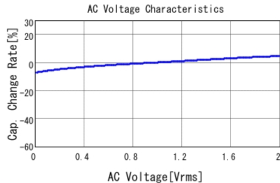
■ GRM033R61E472KA12 C-AC Voltage capchange, DCOV, 25.0d
