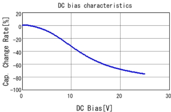
■ GRM033R61E472KA12 C-DC bias capchange, 25.0degC, AC1.
