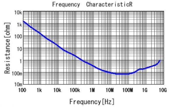
■ GRM033R71A682KA01 R DCOV, 25degC
