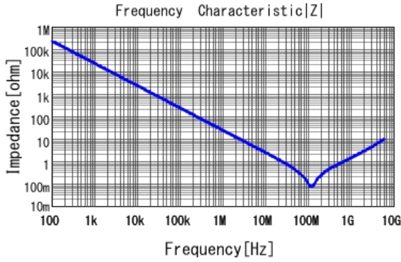
■ GRM033R71A682KA01 |Z| DCOV, 25degC
