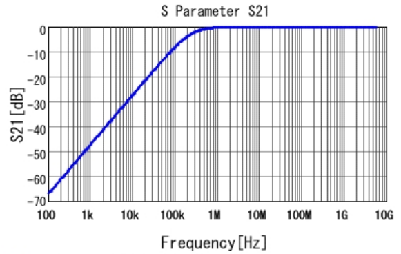
■ GRM033R71A682KA01 S21 DC0V, 25degC
