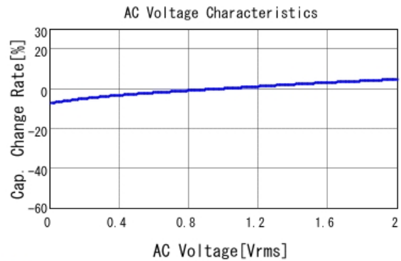
■ GRM033R71A682KA01 C-AC Voltage capchange, DCOV, 25.0d
