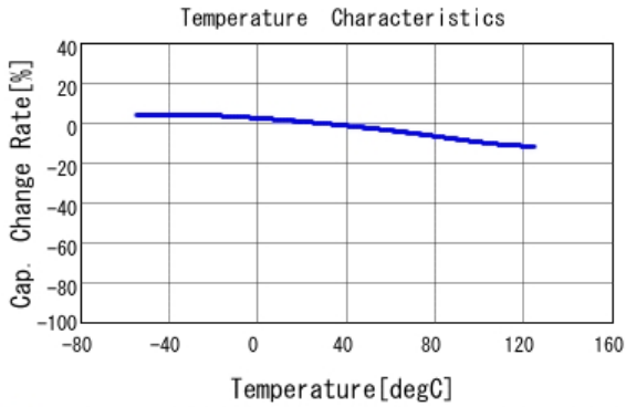
■ GRM033R71A682KA01 C-Temp. capchange, DC0.0V, AC1.0Vrm
