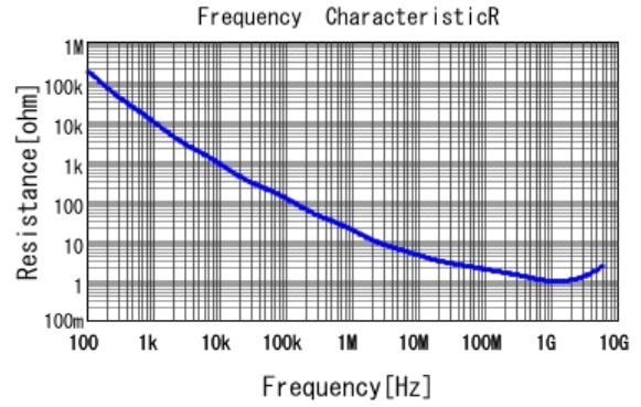
■ GRM033R71C101KA01 R DCOV, 25degC
