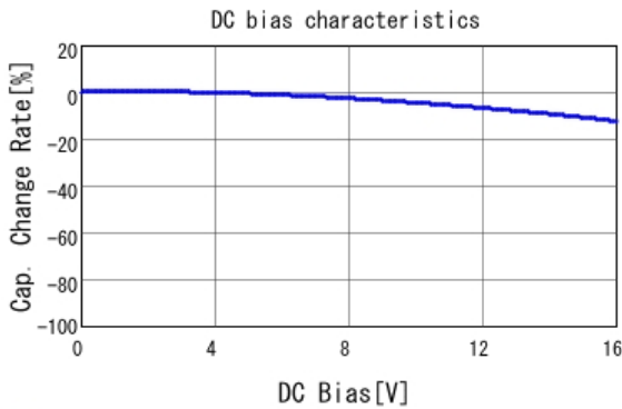
■ GRM033R71C102KA01 C-DC bias capchange, 25.0degC, AC1.
