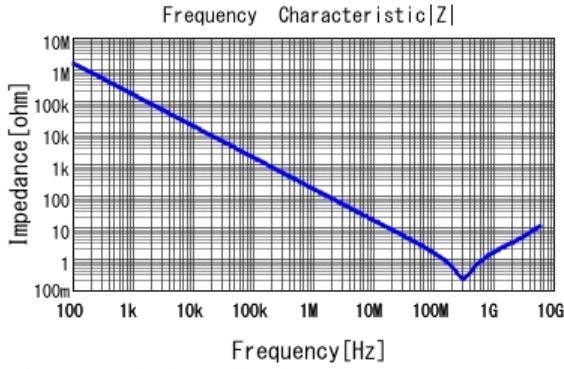
■ GRM033R71C102KA01 |Z| DCOV, 25degC
