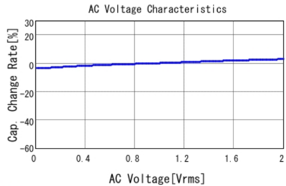
■ GRM033R71C102KA01 C-AC Voltage capchange, DCOV, 25.0d
