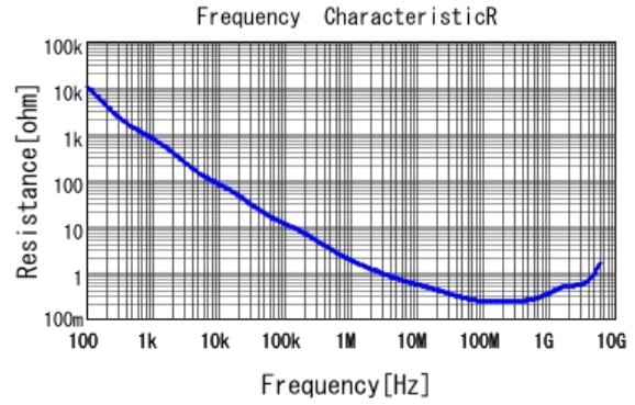
■ GRM033R71C102KA01 R DCOV, 25degC
