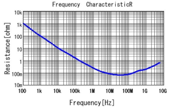
■ GRM033R71C103KE14 R DCOV, 25degC
