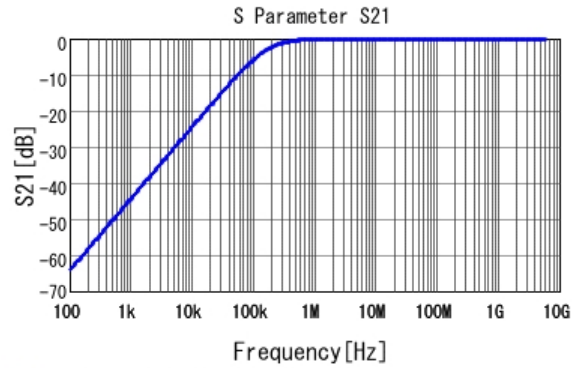
■ GRM033R71C103KE14 S21 DC0V, 25degC
